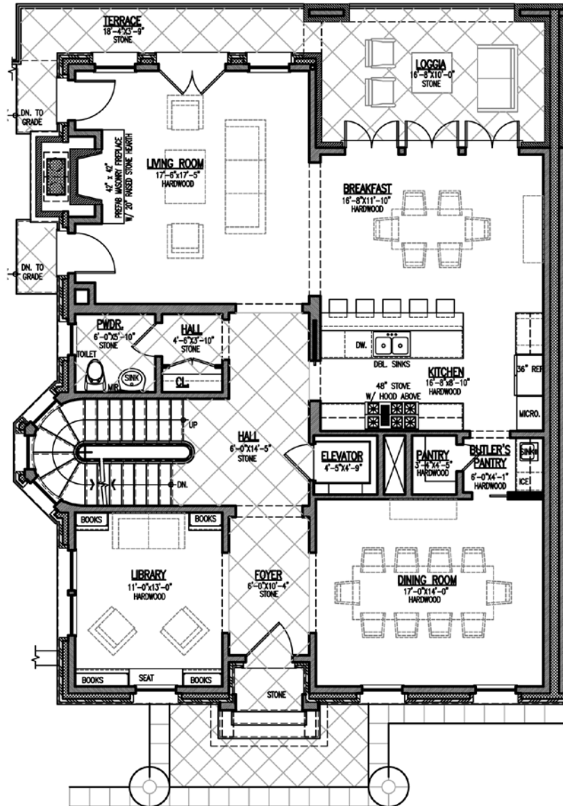
Main Level Heated Area 1,695 Sq. ft.
